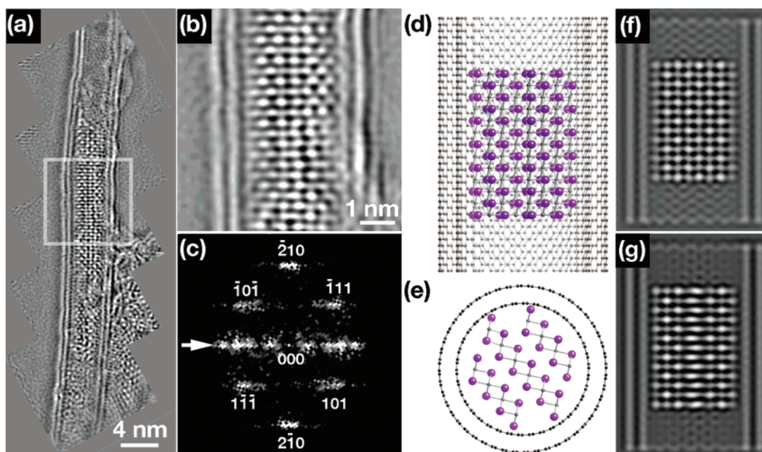
Figure 9. (a and b) Restored HRTEM phase image and detail of a 2.5 nm i.d. DWNT filled continuously with PbI 2 . (c) Power spectrum obtained from the indicated region in a and indexed according to a \langle 121 \rangle projection. (d and e) Side-on and end-on models of the derived model of the PbI 2 @DWNT composites. (f) Multislice simulation of the image phase produced from the model in d. (g) As for d but rotated 5° about the DWNT axis relative to the orientation depicted in e.
