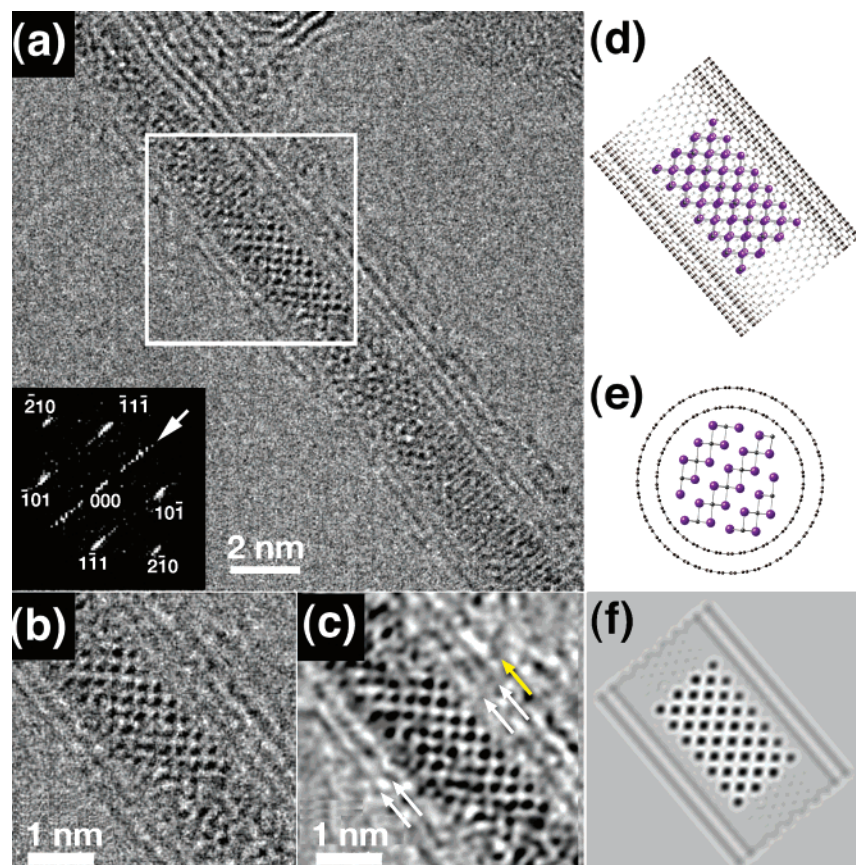
Figure 8. (a) Conventional HRTEM image of a 2.5 nm i.d. DWNT filled continuously with PbI 2 . The inset power spectrum obtained from the indicated region in the main image is indexed according to a \langle 121 \rangle projection. (b and c) Detail and noise-filtered image of the indicated region in a. (d and e) Side-on and end-on models of the derived model of the PbI 2 /DWNT composites. (f) Scherzer defocus image produced from the model in d.
